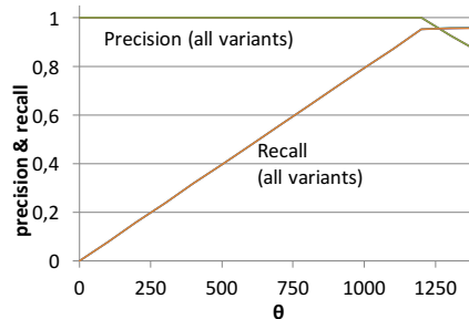
Figure 6: Our method achieves high precision and recall; the corrupted edges are successfully detected. Left: 10% noise; right: 20% noise.
