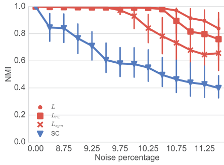
Figure 7: Robustness to noise. Our RSC clearly outperforms spectral clustering.
