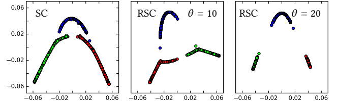
Figure 2: Spectral embeddings for data of Fig. 1 (right). Left: Spectral clustering; middle: RSC with \theta = 10 , right: \theta = 20 . RSC enhances the discrimination of points.
