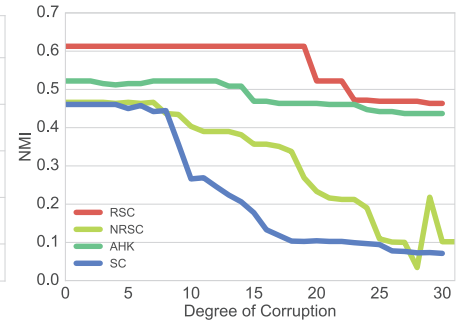
Figure 9: Robustness of all techniques on banknote. RSC is very stable.
