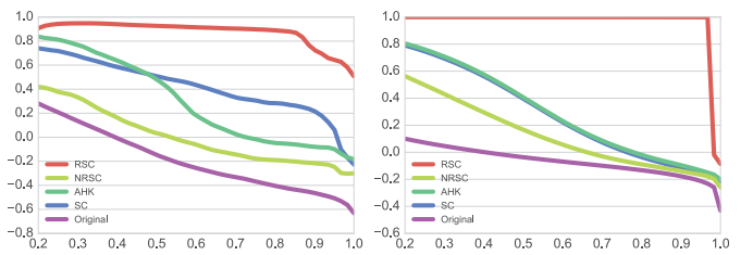
Figure 11: Evaluation of global separation (left: banknote, right: USPS). RSC’s embedding separates the classes well.
