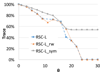
Figure 5: Our method obtains better (lower) trace values (trace of SC=100%)
