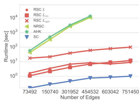
Figure 8: Runtime analysis. RSC scales linear in the number of edges
