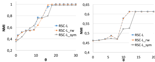
Figure 4: Increasing the sparsity threshold \theta improves the clustering quality. Left: two moons data; right: banknote.
