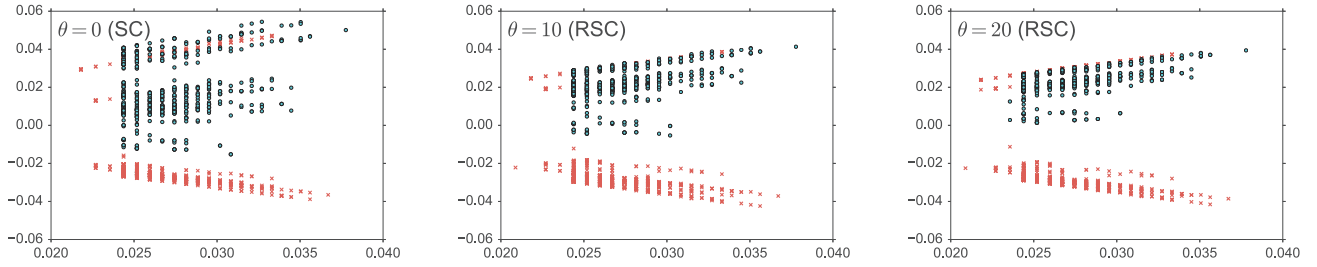
Figure 3: Spectral embedding of banknote data based on L_{sym} . Note that the dataset contains two clusters. Left: Standard spectral clustering; middle & right: Our method ( \theta = 10 and 20 ). The learned embeddings increase the discrimination between the points. The two clusters stand out more clearly.
