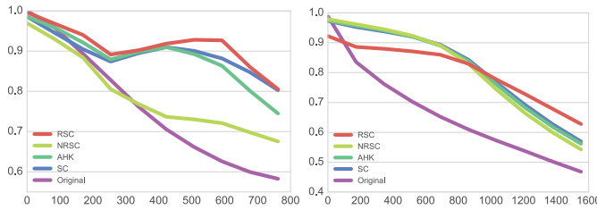
Figure 10: Evaluation of local purity (left: banknote, right: USPS). RSC’s embedding represents the classes well locally.
