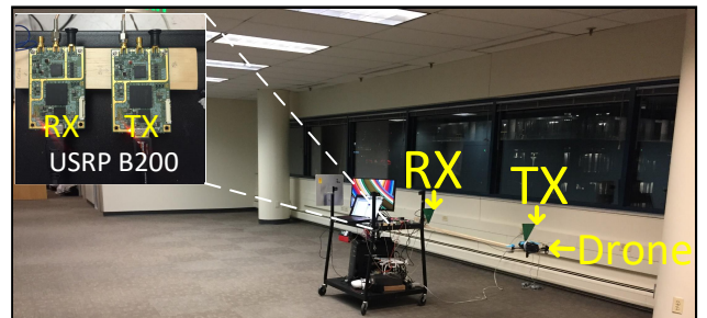
Figure 4: The setup for the indoor environment.
