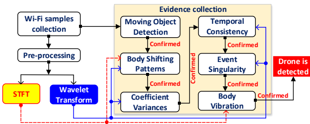
Figure 8: Overview architecture of Matthan.
