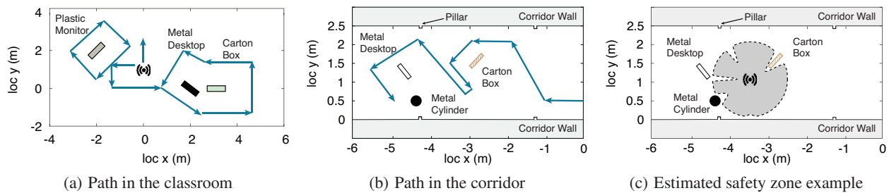
Figure 14: Ulysses navigates in (a) the classroom and (b) the corridor without colliding into objects/walls. In (c) we plot an example of the estimated safety zone (the shaded region) at a specific location.
