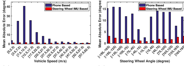
(a) Error distribution with respect to vehicle speed. (b) Error distribution with respect to steering angle.
