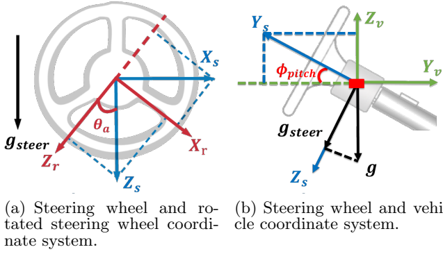
Figure 3: Several coordinate systems and angle estimation.
