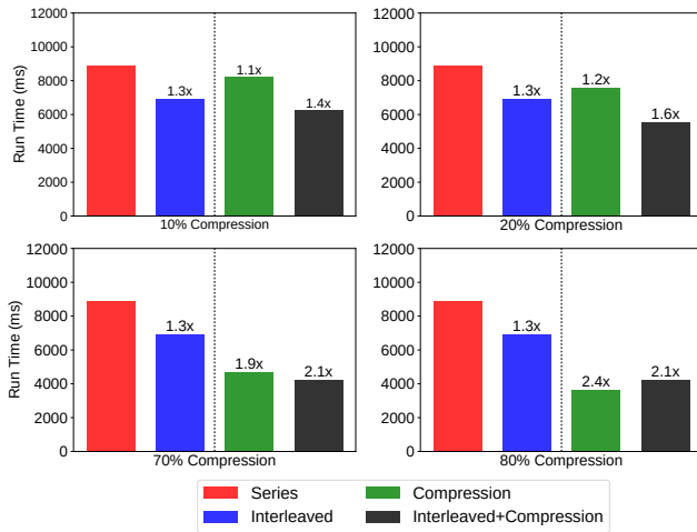
Figure 11: Performance of layer interleaving in combination with model compression approaches. The values on the bars show the latency gain in each case over the baseline Series execution approach.
