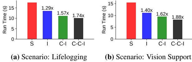
Figure 13: Latency comparison when executing the scenario pipelines on DeepEye. S = Series, I = Interleaved, C-I = Caching+Interleaved, C-C-I = Compression+Caching+Interleaved
