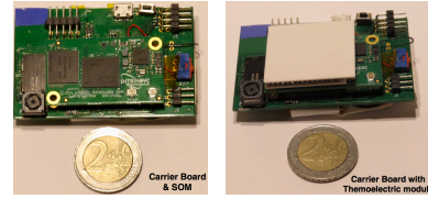
Figure 7: DeepEye Hardware Prototype
