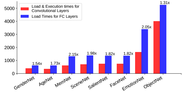
Figure 4: Understanding the bottleneck in deep vision model execution on embedded platforms. Loading model parameters is the single most time consuming task, which was seen across eight different models popular within the computer vision community.
