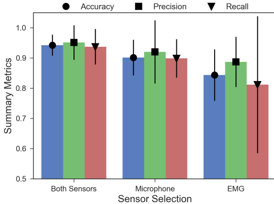
Figure 6: Summary metrics when using contact microphone and EMG, independently and combined (error bars represent standard deviation).
