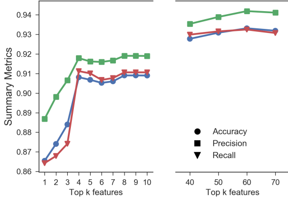
Figure 8: Results when number of features ranged from 1 to 70
