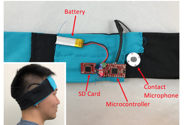
Figure 4: Wearable apparatus
