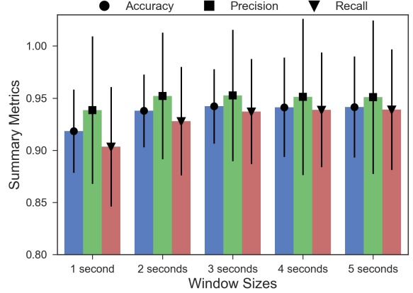
Figure 7: Summary metrics when window size ranges from 1 second to 5 seconds (error bars represent standard deviation)
