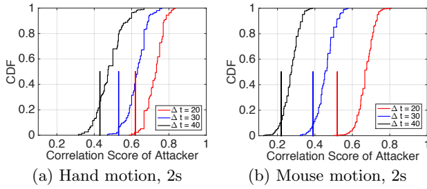
Figure 3: CDF of correlation score by attacker
