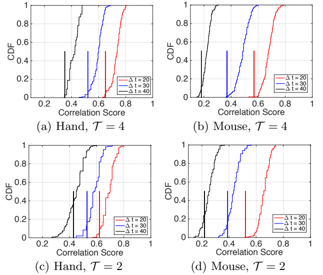
Figure 2: CDF of correlation scores
