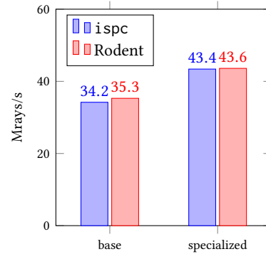
Fig. 3. Shading performance on an i7 6700K for the simple shader described in Section 5.3 implemented using Rodent and iSpC (higher is better). Specialization is done manually in the iSpC version.
