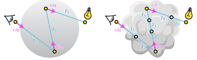
Fig. 2. Recursive estimation of the VRE can be done via a series of direction, \omega , and distance, t , sampling decisions. With the classical formulation (3), this is possible only in (piecewise) simple media, e.g. with linearly varying density (left), where transmittance along rays can be sampled analytically. To enable unbiased light transport estimation in general heterogeneous media, the null-scattering formulation (9) augments the medium with fictitious scattering matter to obtain a combined medium where the transmittance between two scattering events (real or fictitious) is analytically sampleable (right).
