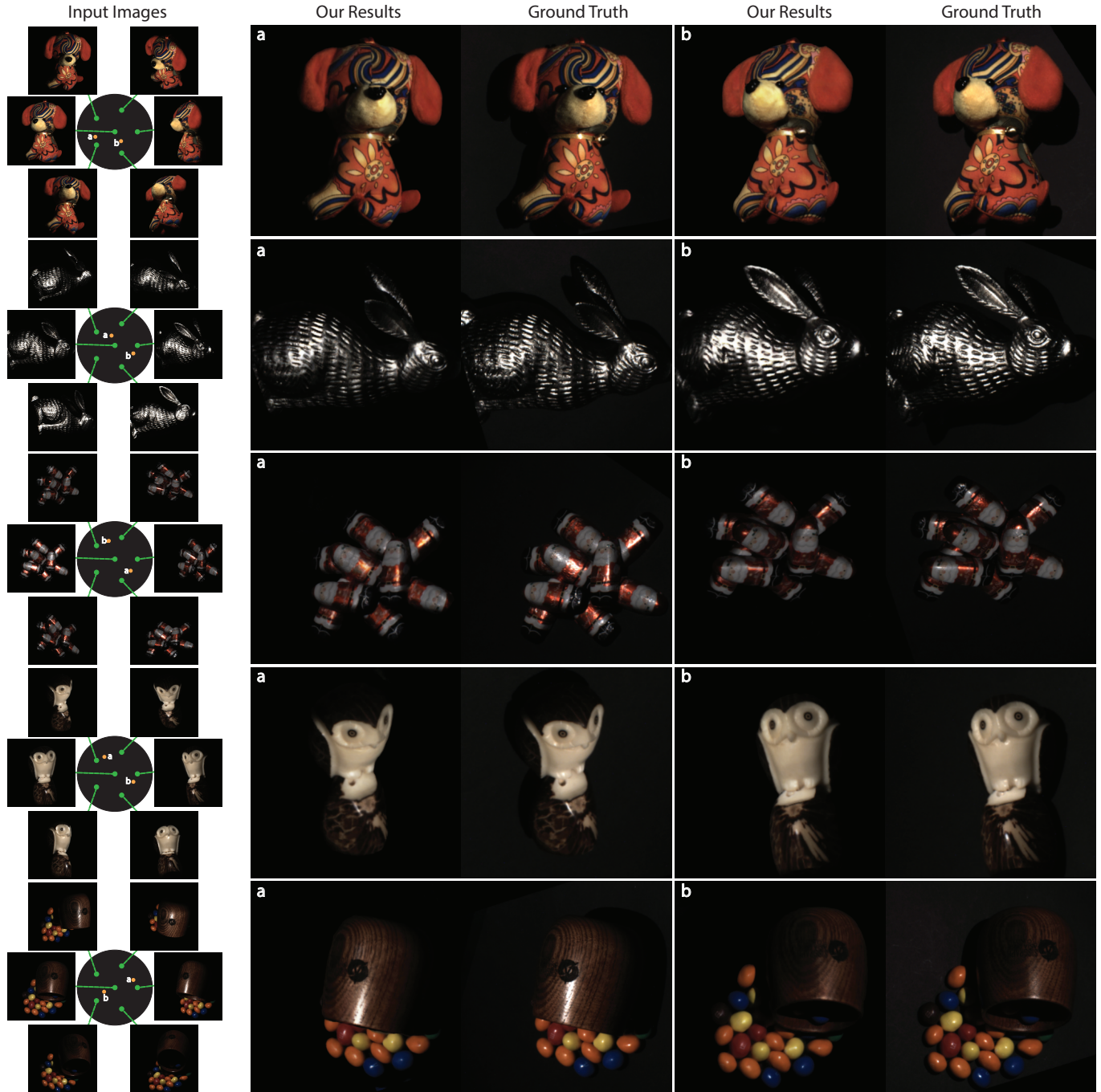
Fig. 10. Novel view synthesis results from our single-light network on real scenes. For each scene, we show two novel view synthesis results (second and fourth columns) compared with captured ground truth images (third and fifth columns), whose viewing directions are marked in yellow with corresponding labels (a and b). We also show the inputs in the first column marked with corresponding viewing directions in green.
