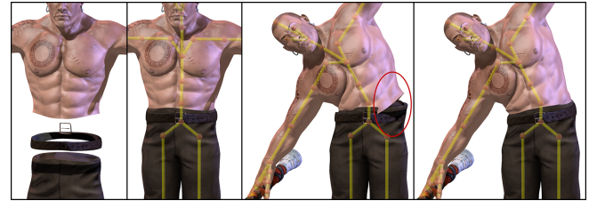
Fig. 6. Our trivial solution to handle models with multiple geometry parts. From left to right: (1) visualization of multiple parts of our character model, (2) the model at rest pose, (3) applying per-part mesh Laplacians breaks the deformation at boundaries of parts, (4) our fix by adding entries to the Laplacian matrix connecting close vertices associated to the same bone.
