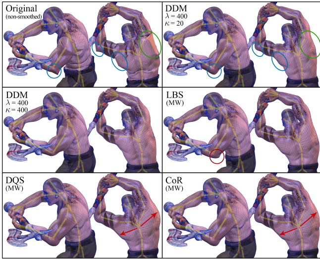
Fig. 9. Further comparison of DDM and other methods on the upper body of a detailed character. DDM is the first direct skinning method that can avoid the indicated bulging artifacts. Also see the accompanying video.
