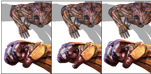
Fig. 7. Local control for different body part sizes. Left: DDM with five iterations and a global step size of 0.5 did not produce smooth deformation on the elbow. Middle: DDM with 100 iterations and a global step size of 0.5 produced good elbow deformation but it over-smoothed the finger deformations. Right: DDM with per-vertex weights (with parameters showed in Table 2) produces pleasing deformation for both elbow and fingers.
