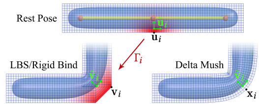
Fig. 2. The core idea of Direct Delta Mush schemes. The accumulated affect of iterated Laplacian smoothing is captured in a per-vertex weight mask (column \mathcal{B}_i , red color gradient) that if applied to the undeformed geometry produces the equivalent of the iteratively smoothed result (inner blue geometry). These weights are used to solve for the local coordinate transformation \Gamma_i which is defined as the best rigid transformation to align the local patch (red regions) from the rest pose to the LBS deformed pose, a.k.a. a form of Weighted Procrustes problem. The delta between \mathbf{u}_i and \tilde{\mathbf{u}}_i is also transformed and added to the smoothed deformed position \tilde{\mathbf{v}}_i , producing the final vertex position \mathbf{x}_i .
