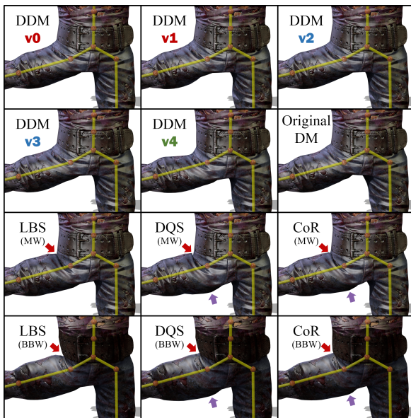
Fig. 10. A comparison of deformation at the hip joint: DM-based methods, including original DM and four variants of our DDM ( v0 , v1 , v2 , and v3 ), produce no clefts or fold-over due to the negative bulging. The clefts of other methods are indicated by red arrows. Notice that DDM v4 has only one single weight for translation so it “cheats” by expanding the inner thigh (purple arrow) as happens in quaternion-based methods (DQS and CoR). The bends of DQS and CoR are more extreme so they create bulges (purple arrows). The original DM is setup with 100 iterations and step size of 0.5.
