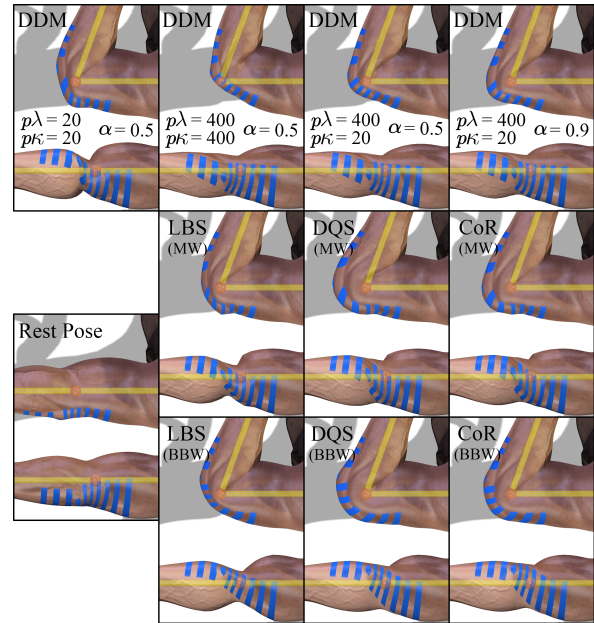
Fig. 8. Our DDM with different configurations (top row): using higher rotation smoothing step size \lambda produces smoother deformation when twisting the joint, while using lower translation smoothing step size \kappa produces more rigid deformation when bending the joint, similar to other skinning methods. Adjusting the blending weight \alpha results in simultaneous rigid bend and smooth twist and mimics the sliding and stretching of skin on top of a knuckle. Notice how DDM with \alpha = 0.5 or \alpha = 0.9 produces more uniform skin stretching. Because our translation blending (§3.3) does not affect rotation, the smoothing effect on twisting does not change with different translation smoothing step size or blending weight (last three figures on the top row). Comparisons with other methods are shown in the bottom row. Without the independent control provided by DDM, other methods have to compromise between bending deformation quality or twisting deformation quality, typically resulting in suboptimal quality for both.
