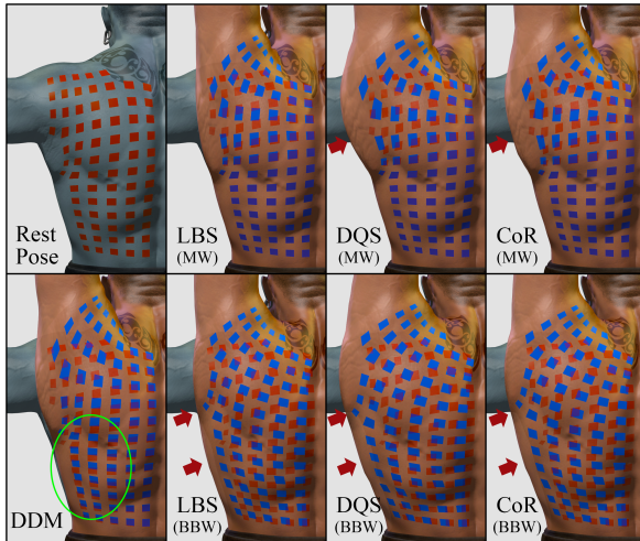
Fig. 12. DDM can produce a skin sliding effect on the mid-lower back without the accompanying bulges caused by long-range weights in other methods.
