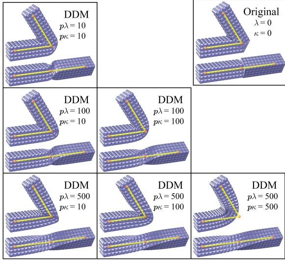
Fig. 4. Our extension: the original DM uses a single control for smoothness, which can only produce deformations similar to figures on the diagonal (with p\lambda = p\kappa ). Our extension allows blending different rotation smoothness (controlled by p\lambda ) and translation smoothness (controlled by p\kappa ). This unique translation blending does not affect rotation (proven in Appendix C) which makes authoring less challenging. In the last row, changing p\kappa does not change the twist deformation. The bottom left corner with p\lambda = 500 , p\kappa = 10 is a good pattern for elbow deformation, which mimics the skin sliding on top of a knuckle.
