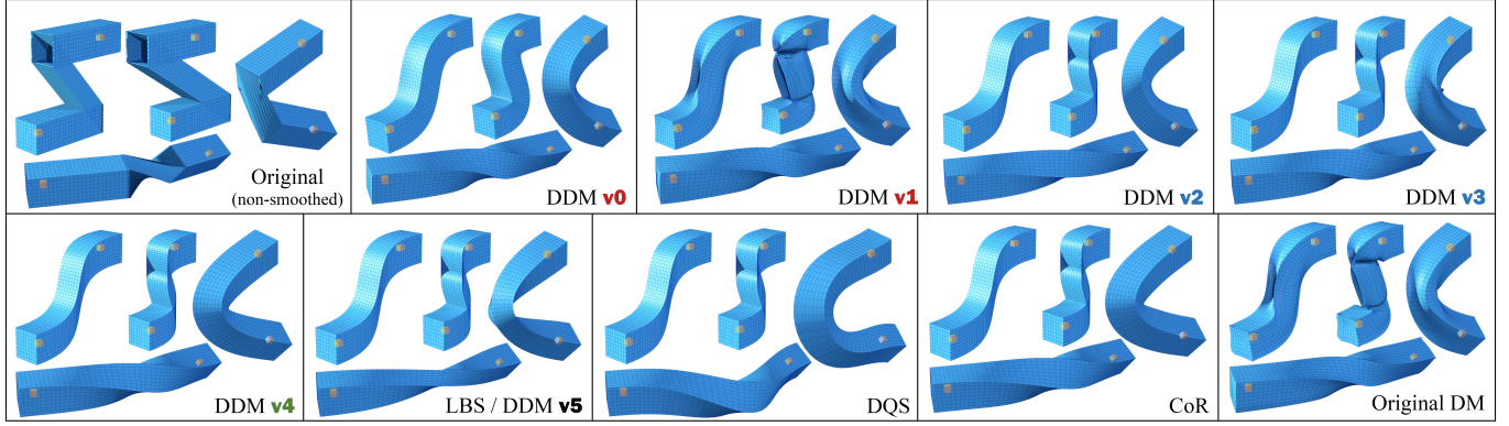
Fig. 5. Different variants of our DDM. The bar's deformation is controlled by two disconnected bones (yellow). Variants with higher number use less resources and produce more deformation artifacts. Run time deformations of some DDM variants are equivalent to previous skinning models: DDM v1 is equivalent to the original DM, DDM v4 is equivalent to CoR, and DDM v5 is equivalent to LBS.
