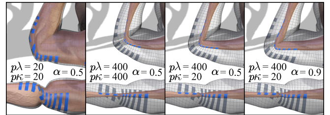
Fig. 11. Volume preservation behavior of the model (gray wireframed) depends on the volume of the mush (color shaded) at the rest pose. Leftmost: with low smoothness p\lambda , the mush does not shrink much, but some of this remaining volume can be lost with deformation. Middle and right: with high smoothness p\lambda , the mush shrinks to a rod-like shape with near zero volume and this cannot be further reduced by deformation. Bending deformation can be controlled by changing the translation smoothness p\kappa and its blending weight \alpha .
