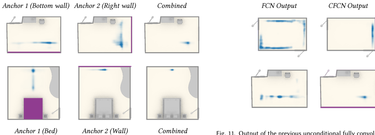
Fig. 10. Combining multiple anchor-relative location distributions into one global distribution. The anchor object is highlighted in purple. Note how the product of the two anchor-relative distributions leaves an unambiguous signal that the bed should be in the corner ( top row ) and that the TV stand should be directly across from the bed ( bottom row ).
