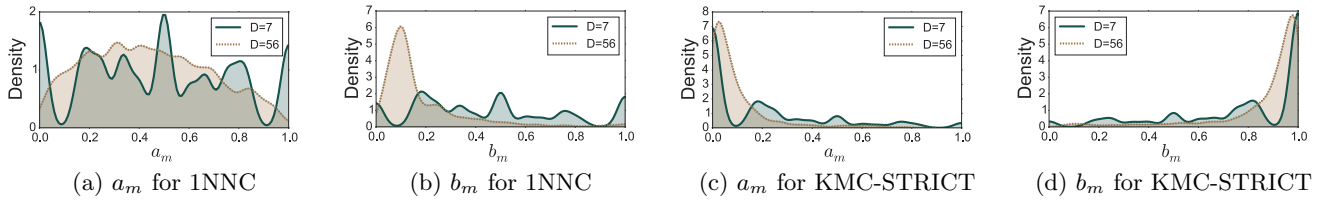
Figure 5: Distribution of a_m and b_m of highly active users (estimated with kernel density estimator)
