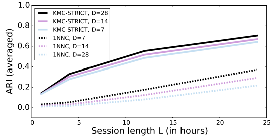
Figure 6: Averaged ARI for varying session length L
