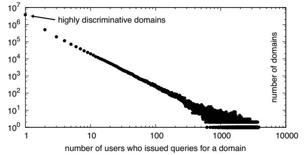
Figure 3: Discriminativens of domains (original dataset)
