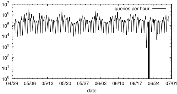
Figure 2: Time series of hourly query rate
