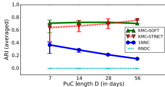
Figure 4: Averaged ARI for varying PuC length D
