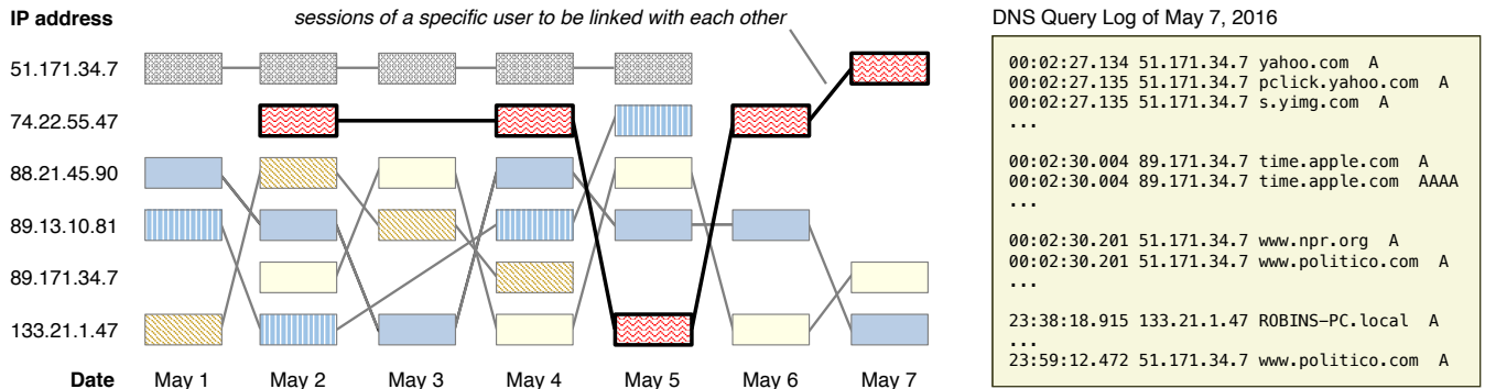
Figure 1: Scenario and objective of behavior-based tracking
