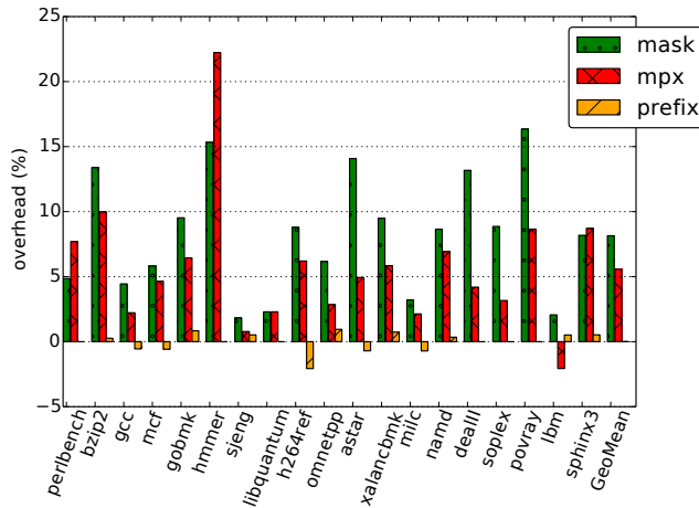
Figure 6: Performance overhead on SPEC CPU2006 for three non-sensitive protection options: masking, Intel MPX, and address override prefix.
