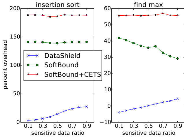
Figure 5: Performance overhead measured on two microbenchmarks when varying the proportion of sensitive to non-sensitive data. More sensitive data leads to higher overhead for DataShield but not for SoftBound + CETS.
