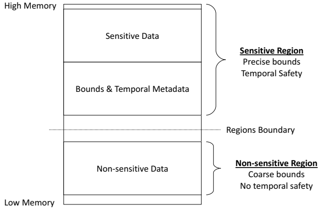
Figure 1: DataShield’s runtime memory layout for sensitive and non-sensitive data. The sensitive region has a strict security policy that leads to instrumentation overhead, and the non-sensitive region has a relaxed security policy with minimal overhead.
