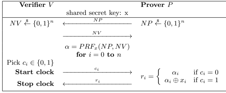
Figure 1: The classical countermeasure against terrorist fraud: if the prover gives both possible responses, such as for instance \alpha_i and \alpha_i \oplus x_i to his accomplice for a given c_i , he leaks one bit of his long-term authentication secret x . Note that PRF is a pseudorandom function keyed with x .
