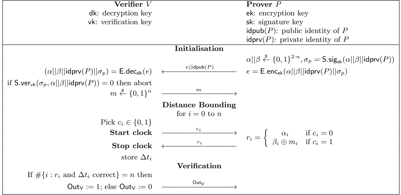
Figure 2: Our generic and provably secure DB construction TREAD built from an IND-CCA2-secure encryption scheme E and an EUF-CMA-secure signature scheme S . The symbol || denotes the concatenation operation.
