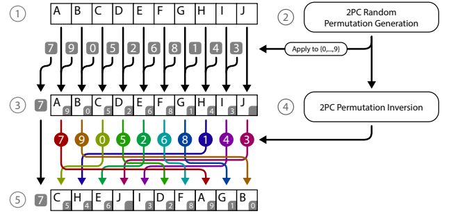
(a) Initialization. The input ① is combined with a random permutation ② which has been shifted left by one place. The result ③ is then permuted according to the inverse of the first permutation ④, resulting in a shuffled linked list ⑤. The leftmost element of the first random permutation ② is retained outside the structure and represents the entry point.
