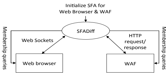
Figure 5: The setup for SFADiff finding differences
