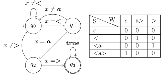
Figure 3: A Symbolic Finite Automaton (SFA) for the regular expression .*<a>.* and the corresponding entries for the S, W sets from the observation table.
