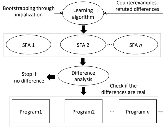
Figure 1: SFADiff architecture
