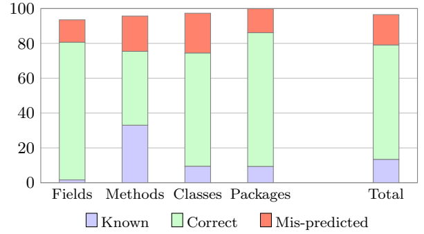
Figure 6: Average percentage of known, correctly predicted, and mis-predicted program elements calculated over the 100 Android applications deobfuscated by DEGUARD.
