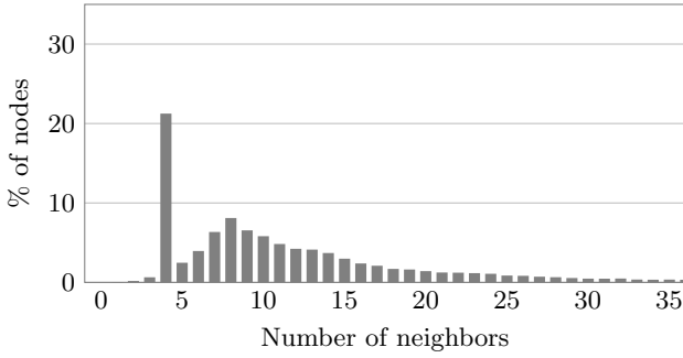
Figure 4: Distribution of total number of neighbors over the 100 ProGuard-obfuscated Android applications.
