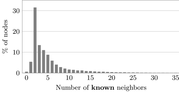
Figure 5: Distribution of known number of neighbors over the 100 ProGuard-obfuscated Android applications.
