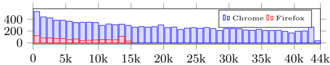
Figure 2: Amount of discoverable browser extensions (y-axis, not stacked) based on extensions’ popularity rank (x-axis)
