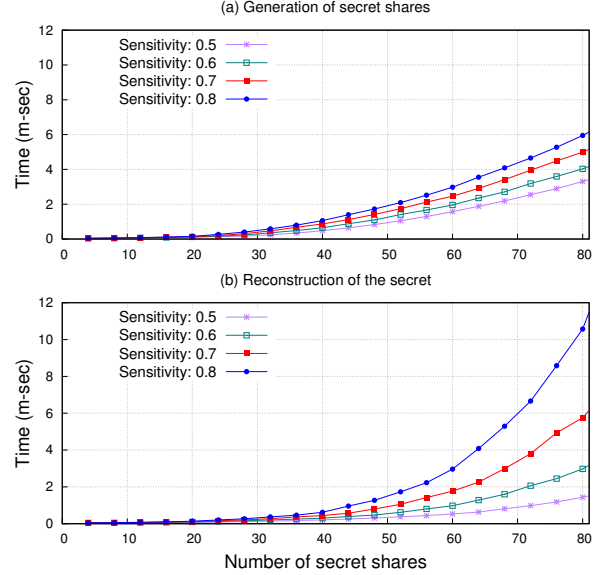
Figure 5: Time overhead for (a) generating a number of secret shares and (b) reconstructing the secret from a sufficient number of shares, with regards to object's sensitivity level.
