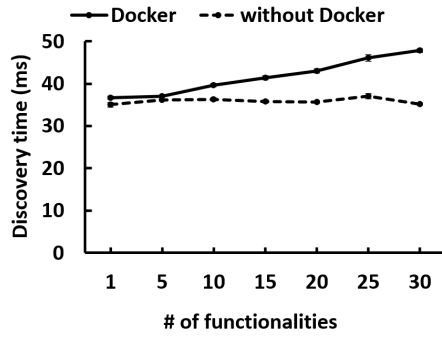
Figure 8: Discovery time according to the number of functionalities
