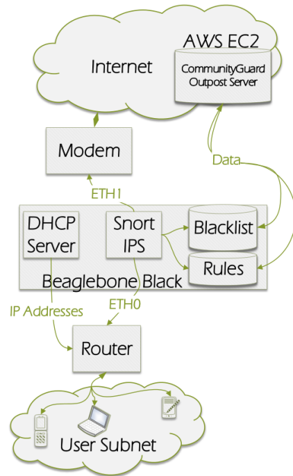
Figure 2: Prototype Overview.
