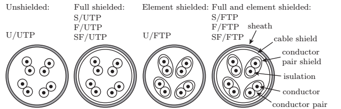
Figure 3: Differently shielded twisted-pair cables
