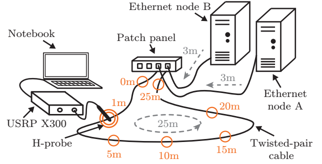
Figure 1: Lab environment for the eavesdropping attack evaluation
