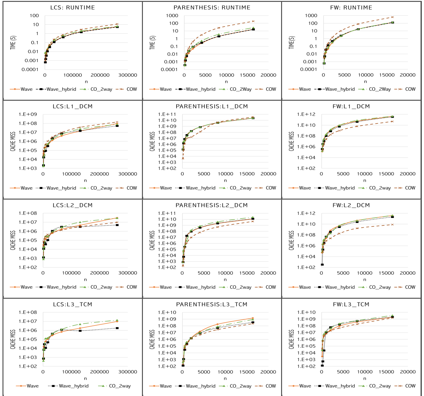
Figure 4: Runtimes and cache misses in three levels of caches for classic 2-way recursive divide-and-conquer, COW and recursive wavefront algorithms for LCS, Parenthesis and 2D FW-APSP Problems. All programs were run on 16 core machines in Stampede. All implementations used Cilk Plus’s work-stealing scheduler.
