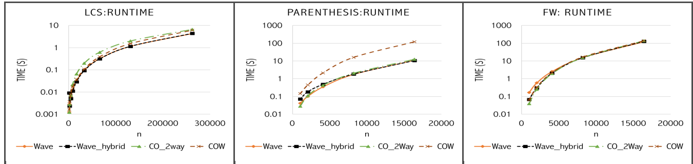
Figure 6: Runtimes for classic 2-way recursive divide-and-conquer, COW and recursive wavefront algorithms for LCS, Parenthesis and 2D FW-APSP. All programs were run on 24 core machines in Comet. All implementations used cilk plus's work-stealing scheduler.
