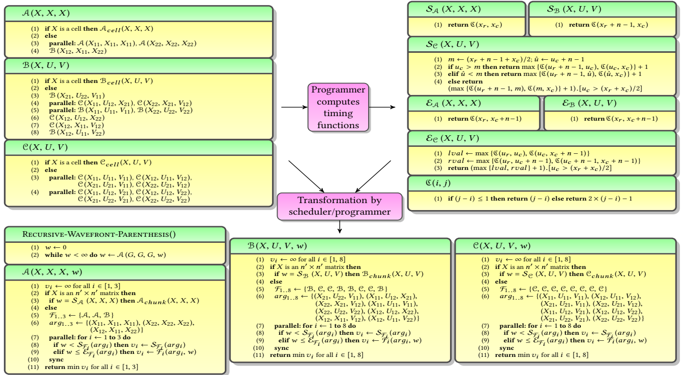
Figure 2: TOP: The programmer derives the timing functions (top-right) from a given standard 2-way recursive divide-and-conquer DP algorithm for the parenthesis problem (top-left). A region Z has its top-left corner at (z_r, z_c) and is of size n \times n . BOTTOM: A recursive divide-and-conquer wavefront algorithm is generated for the parenthesis problem. The programmer derives the algorithm if work-stealing scheduler (see Section 4.1) is used and the scheduler derives the algorithm if W-SB scheduler (see Section 4.2) is used. The algorithm makes use of the timing functions derived by the programmer.
