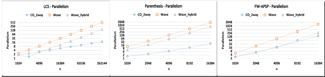
Figure 5: Projected scalability of new recursive wavefront algorithms by Cilkview Scalability Analyzer. The numbers denote till how many cores the implementation should scale linearly.
