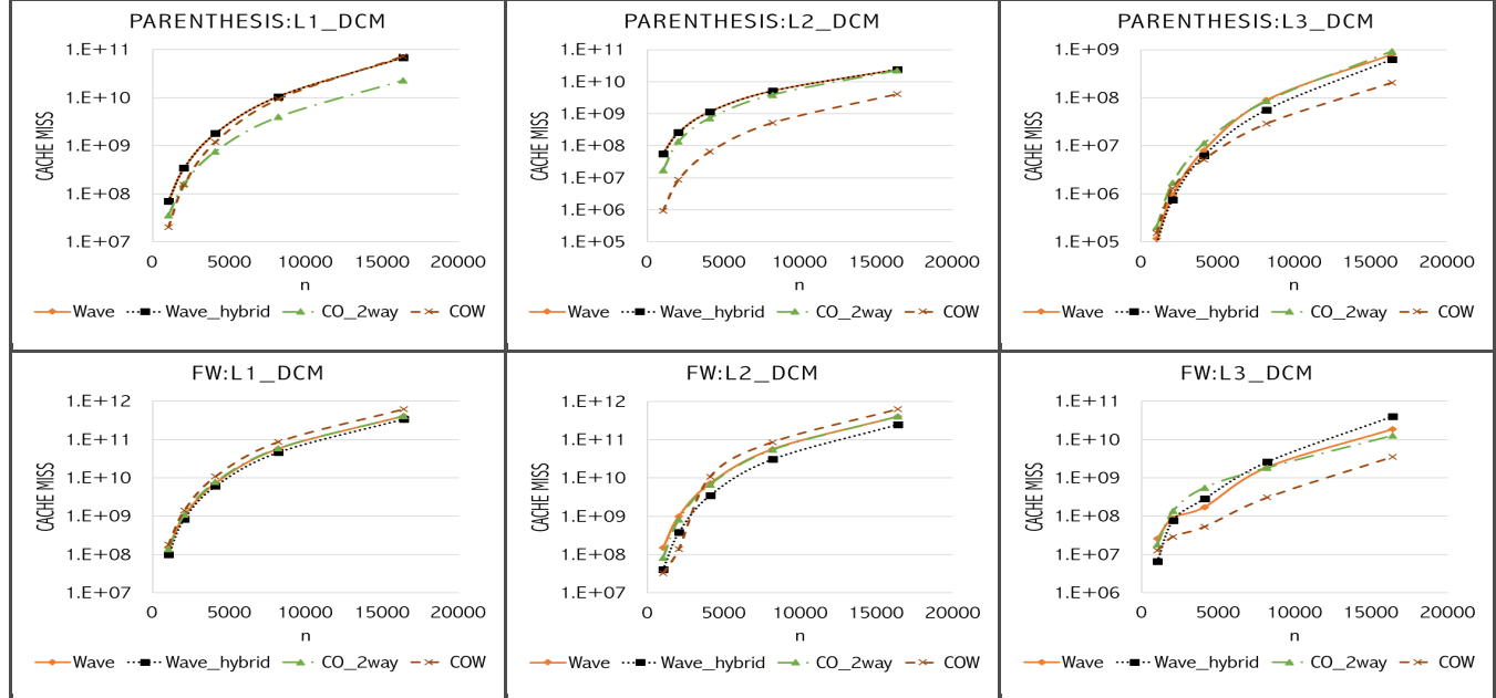
Figure 7: Cache misses in three levels of caches for classic 2-way recursive divide-and-conquer, COW and recursive wavefront algorithms for Parenthesis and 2D FW-APSP. All programs were run on 24 core machines in Comet. All implementations used cilk plus's work-stealing scheduler.
