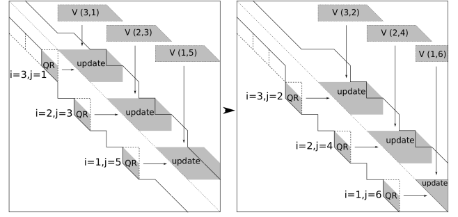
Figure 2: QR factorizations and updates in iterations (i, j) \in \{(3, 1), (2, 3), (1, 5)\} (left) and (i, j) \in \{(3, 2), (2, 4), (1, 6)\} (right) of Algorithm 4.1 with k = 2 . These two sets of iterations are executed concurrently by processor groups \hat{\Pi}_1, \hat{\Pi}_3, and \hat{\Pi}_5 (left) and \hat{\Pi}_2, \hat{\Pi}_4, and \hat{\Pi}_6 (right), respectively. Only the unique part of the trailing matrix update is shown, while the pseudocode performs both symmetric reflections of it. Each matrix V is labeled with the iteration in which it is computed.
