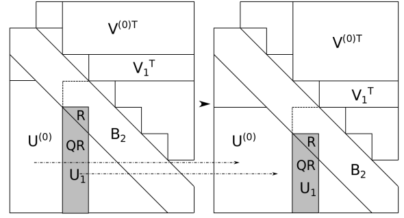
Figure 1: A depiction of matrices used in Algorithm 4.1 for two subsequent recursive steps.
