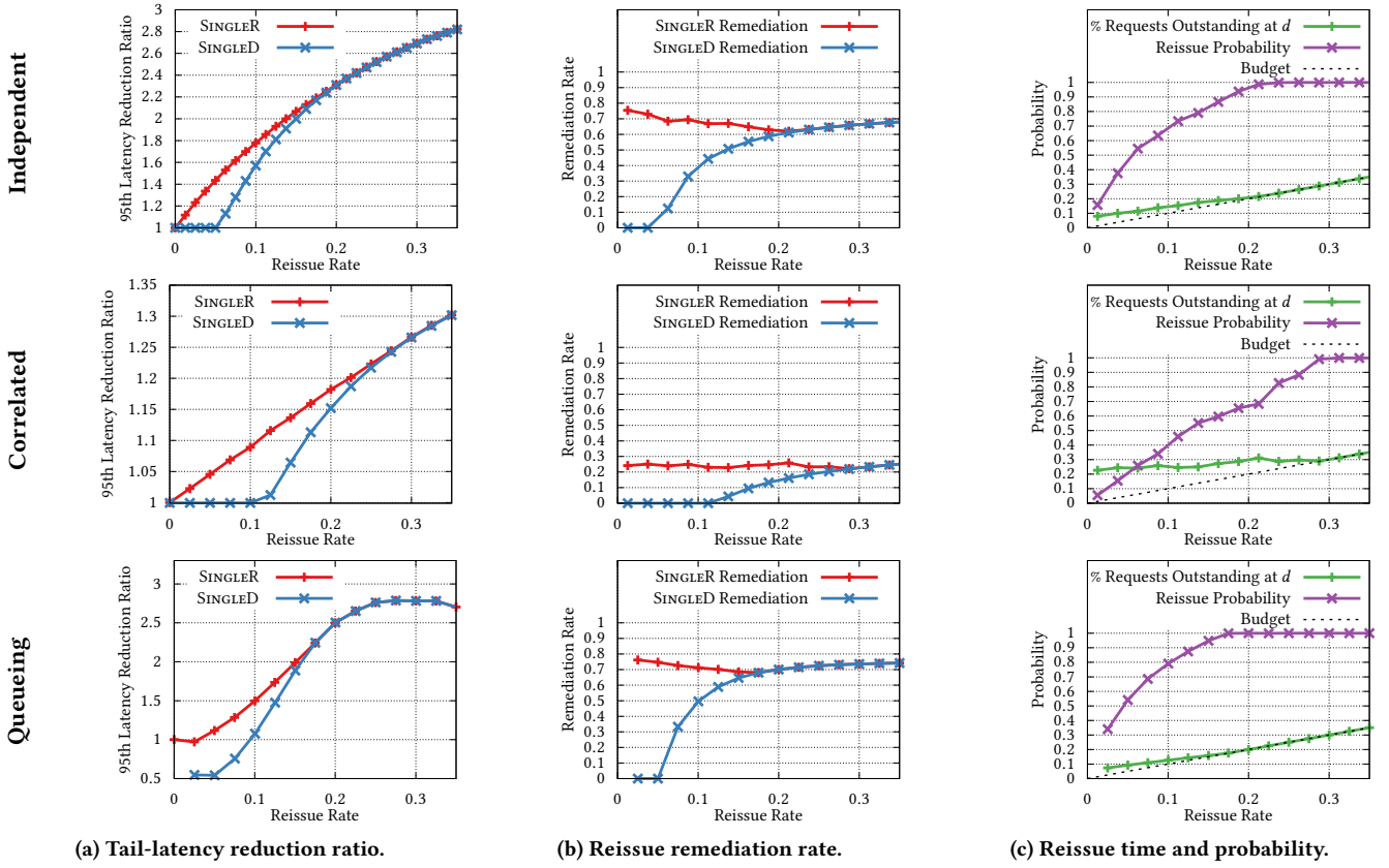
Figure 3: Simulation results for SINGLER and SINGLED policies with varied reissue budgets on three simulated workloads: Independent , Correlated , and Queueing .
