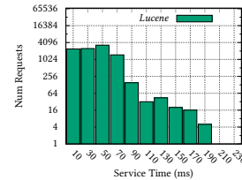
Figure 9: Service time distributions for the Redis set-intersection and Lucene search workloads.
