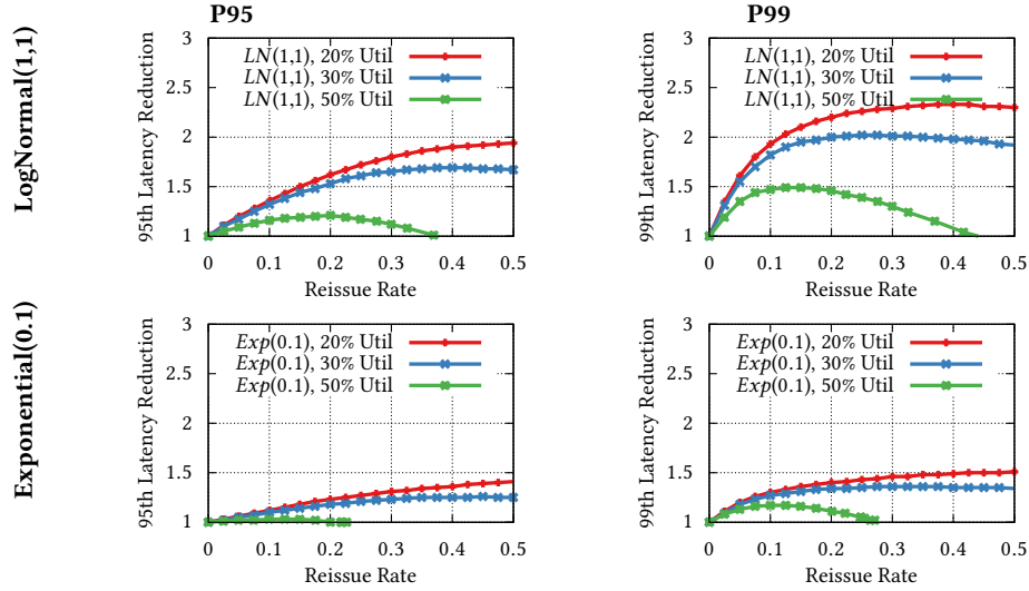
Figure 6: The 95th percentile tail-latency P_{95} and the 99th percentile tail-latency P_{99} for \text{Exp}(0.1) and \text{LogNormal}(1,1) distributions with varied reissue rates and system utilization.
