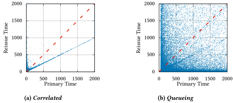
Figure 4: Response-time correlations between primary and reissue requests on the Correlated and Queueing workloads. The service-time X of the primary request is drawn from a Pareto distribution with shape 1.1 and mode 2. The service-time Y of a reissued request is drawn from Y = rX + Z , where x is the observed service-time of the primary request, Z is drawn from a Pareto distribution with shape 1.1 and mode 2, and r = 0.5 .
