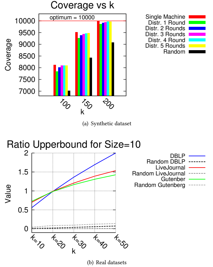
Figure 1: Coverage maximization
