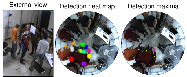
Figure 5: Color-coded joint-location detections on the Crowded sequence. For crowded scenes (left), detections can be multi-modal (center). However, the maximum (right) lies on the user. We exclude knee, hand and ankle locations for clearer visualization.
