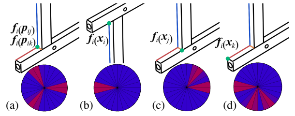
Figure 6: HO features at different locations in a diagram. Features are computed in the local frame of u_i . (a) The graph edges (u_i, u_j) and (u_i, u_k) have the same local features at p_{ij} (here p_{ik} is the same point as p_{ij} ). (b-d) The context features at x_i , x_j and x_k , which are the far ends of paths connecting to p_{ij} , help distinguish (u_i, u_j) from (u_i, u_k) .
