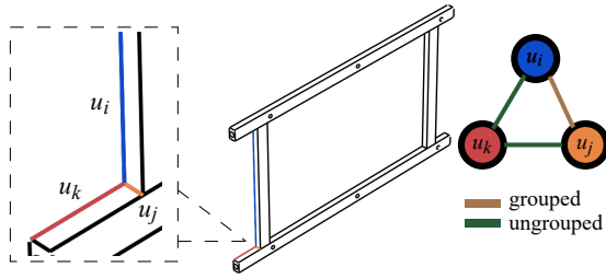
Figure 5: A graph is built from vector graphics primitives. The paths (the blue, yellow and red curves) corresponding to u_i , u_j and u_k connect at the same point, but the graph edges (u_i, u_j) , (u_i, u_k) , (u_j, u_k) should be grouped differently, as they represent edges of different furniture parts.
