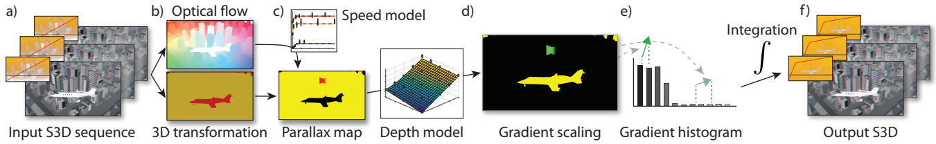
Figure 6: Our disparity mapping algorithm. Optical flow and 3D transformations (b) are extracted for the input S3D sequence (a) and used together with our relative motion model to predict perceptibility of motion parallax in the X and Y directions (c). Our model of perceived depth is then sampled to estimate necessary scaling of each disparity gradient (d). Scaled gradients are accumulated in a histogram (e) and integrated to construct a new mapping curve that is applied to produce the final S3D content (f).
