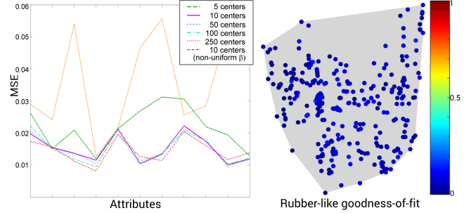
Figure 5: Left: Fitting error (MSE) for our attributes (x-axis). The curves correspond to different numbers of neurons of the RBFs and for non-uniform \beta values (neuron-varying smoothness of the Gaussians); we choose 10 neurons. Right: Mean distances between values predicted by our functionals and subjects' answers for the attribute rubber-like for each BRDF. The low values indicate that our RBFs fit users' opinions well in all regions of the space, and confirm the adequacy of the use of the MOS in their computation.
