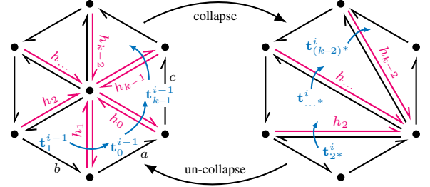
Figure 7: The half edge collapse operator removes a vertex and three pairs of incident half edges while reconnecting the remaining incident half edges to one of its adjacent vertices. Consequently, the inverse collapse operator updates the parametrization of the half edges pointing to the removed vertex and of those half edges that were removed. In addition, consistent transition functions for the three removed edges are computed.
