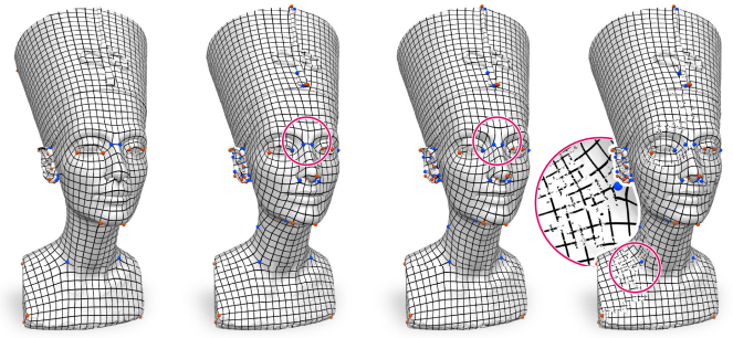
Figure 8: Our pipeline used with (from left to right) [Ebke et al. 2014], [Bommes et al. 2009], [Kälberer et al. 2007] and a seamless parametrization (without integer rounding of translations and singularity parameters), each computed with the same set of alignment constraints. The magnification shows the fragmentation of the chart atlas (which can be defragmented if desired, cf. Section 6.5).
