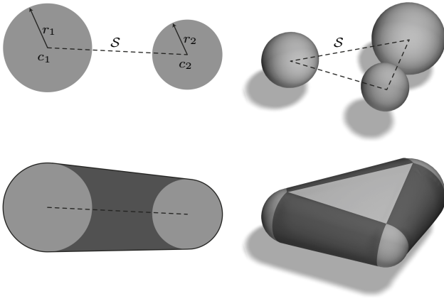
Figure 3: The sphere-mesh skeleton S identifies sphere positions and radii. The surface of the object is obtained as the convex-hull of the spheres on the vertices of the skeleton. Sphere-meshes can be rendered through GPU ray-tracing, or by meshing the zero-crossing of their implicit function; see Eq. 1.
