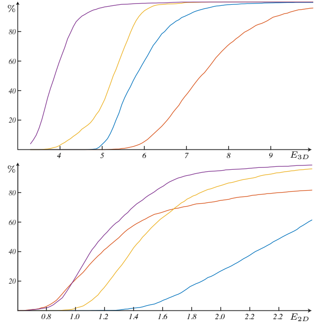
Figure 15: Aggregated errors are reported for the tracking sequences in Figure 14. These aggregated measures reveal a significant improvement in tracking precision; see legend in Figure 14.
