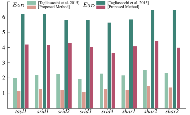
Figure 17: Average 2D/3D tracking performance metrics of the proposed method compared to [Tagliasacchi et al. 2015]. In the additional material we report error plots through time for the aggregated data above.
