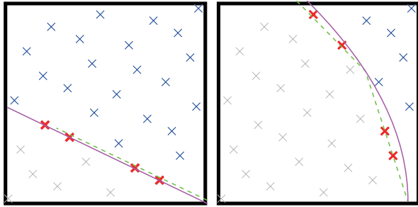
Figure 12: Two example pixels. Incorrect samples are shown as red \times . The solid purple curves show the correct path boundary, and the green dashed lines show the line segments corresponding to the actually fetched mask table entries.
