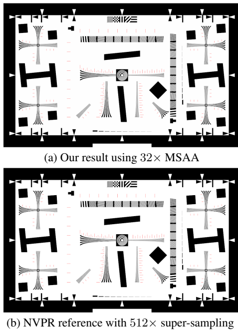
Figure 14: The Reschart image rendered at its original 1024\times 624 resolution. The reference image is generated by down-sampling a 4\times 4 larger image rendered using NVPR with 32\times MSAA.
