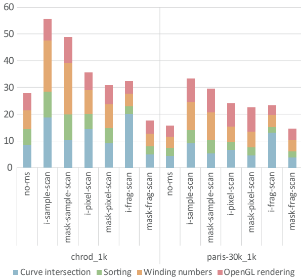
Figure 16: Scanline comparison time break down in milliseconds. We show the performance differences among several implementation variants of our algorithm.
