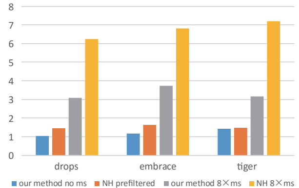
Figure 11: Rendering time of our method and NH in millisecond. We compare our non-multisampling configuration with NH’s pre-filtered rendering mode, and also compare the two methods with 8\times multisampling.
