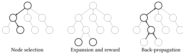
Fig. 5. Exploration mechanism by Monte Carlo Tree Search (after [Browne et al. 2012]). A node is first selected using a tree policy (section 4.1). New nodes are then added (section 4.2) and their corresponding energy are computed (section 4.3). The energy of the new nodes is back-propagated to their parent node to discourage exploring bad configurations (section 4.4).
