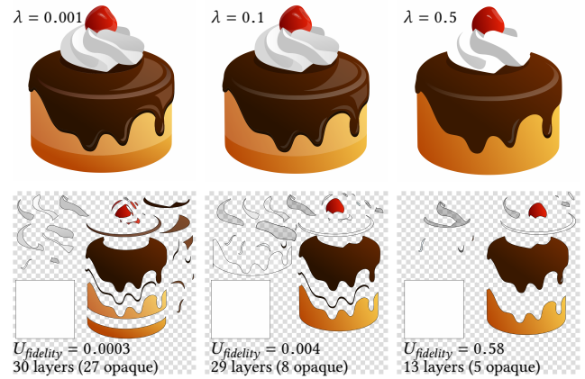
Fig. 9. Impact of parameter \lambda . A low value of \lambda favors accurate reproduction of the input, but produces a decomposition dominated by opaque layers (left). Increasing \lambda turns many of the opaque layers semi-transparent (middle). A high value reduces the number of layers, at the price of missing details (right). Cake by vectorsme on openclipart.org
