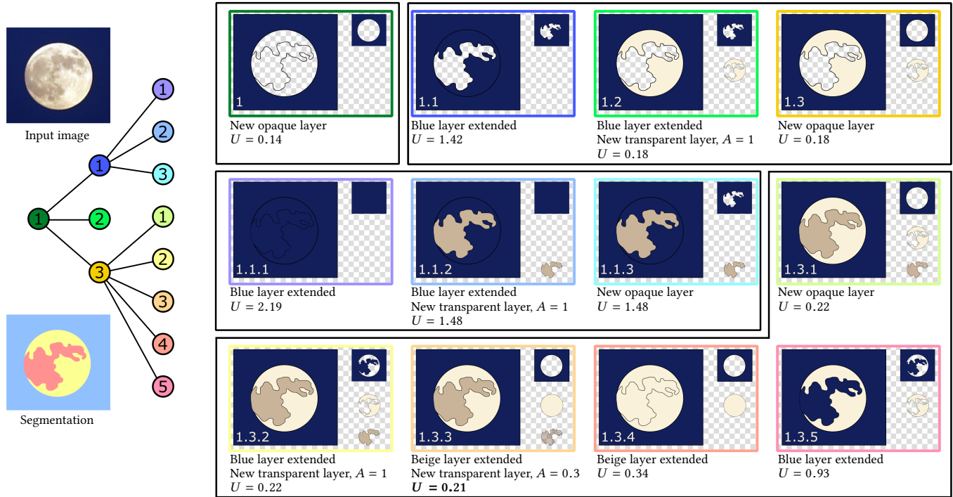
Fig. 4. Overview of our exploration mechanism on a simple example. Given an input image and its region segmentation, we cast the exploration of the solution space as a tree search. Each node of the tree corresponds to an intermediate solution where only a subset of the regions has been decomposed. Each branch of the tree expands an intermediate solution by adding a region to the decomposition. The new region can be assigned to one or several existing layers, as well as to a new layer. Leafs of the tree correspond to complete decompositions. We use Monte Carlo Tree Search to quickly reach low-energy leaves. In this example, the best solution is reached at leaf 1.3.3, where the moon is represented as an opaque beige layer with a semi-transparent brown layer on top. Note that in some configurations, such as node 1.2, a region can be assigned to a new semi-transparent layer which receives an opacity value of 1 after optimization. We convert such layers to opaque when this situation occurs. Moon by stux on pixabay.com
