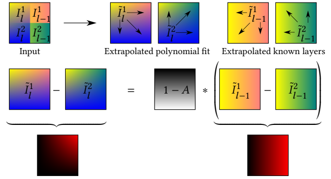
Fig. 7. Derivation of the opacity of a new layer at an X-junction. Let us assume that the new layer is shared by the two regions I_l^1 and I_l^2 . Furthermore, region I_l^1 shares all of its other layers with region I_{l-1}^1 , while region I_l^2 shares all of its other layers with region I_{l-1}^2 . We exploit this redundancy to deduce the opacity of layer l . We first extend each region over the other regions to know their values at each pixel (top). Regions I_{l-1}^1 and I_{l-1}^2 are trivially extended since their layers are known and have a linear form. We extend regions I_l^1 and I_l^2 by fitting a polynomial on their pixel colors. We can then compute a per-pixel opacity A by simple arithmetic (bottom).
