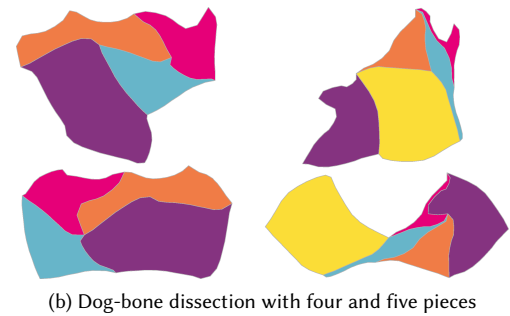
(b) Dog-bone dissection with four and five pieces
