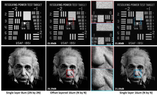
Fig. 5. Synthetic results of the sub-cell offset design. The images are reconstructed from a single DOE with a cell size of 8\mu\text{m} (left column), two DOEs with a cell size of 16\mu\text{m} that are offset by half a cell (middle), and a single DOE with 16\mu\text{m} cells (right). The PSNR are evaluated. Notice that the images are resampled and integrated over the physical size of 200\mu\text{m} per pixel subject to the angular resolution limit of the human eye at the observation distance of 50\text{cm} . The same setting applies to the followings. (1951 USAF Resolution Chart by MIL-STD-150A Standard, Albert Einstein Photograph by Philippe Halsman)
