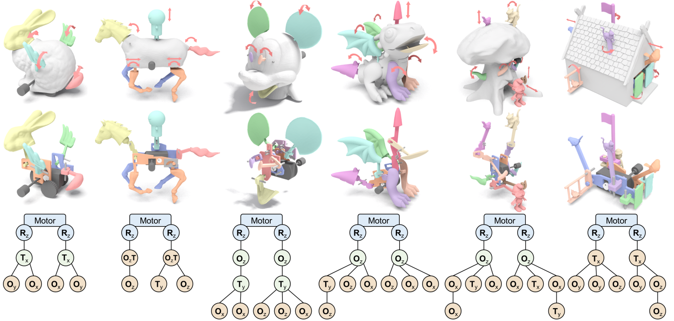
Fig. 14. Some of the wind-up toys produced from our system; from left to right: BUNNY, HORSE, MICKEY, DRAGON, TREE, and HOUSE. From top to bottom: input models and prescribed toy part motions, the optimized wind-up mechanisms, and the associated motion transfer trees, where we color the nodes connected to the external toy parts in orange.
