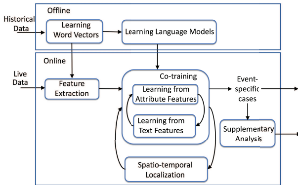
Figure 6: LOTUS System overview
